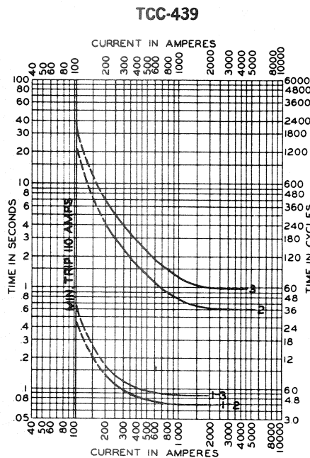
Coil connections are in series. Curves apply to bushing CT ratio of 200:5.
