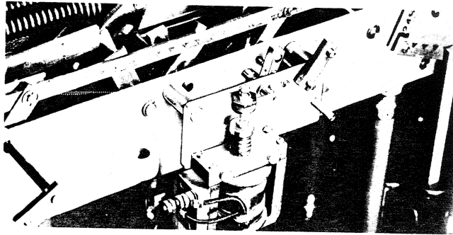
Shunt-trip solenoid mechanism.
