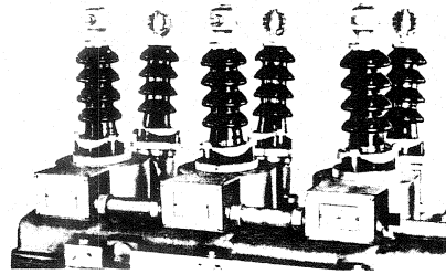
BUSHING CURRENT TRANSFORMERS
