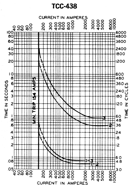
Coil connections are in series. Curves apply to bushing CT ratios of 300:5 and 600:5; they can be indexed to other minimum-trip settings of 205, 247, or 300 amperes.
