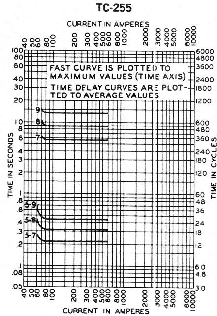
Definite ground-trip TCC's with KA510R solenoids.
