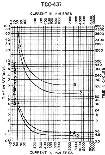
Coil connections are in series. Curves apply to bushing CT ratio of 100:5.
