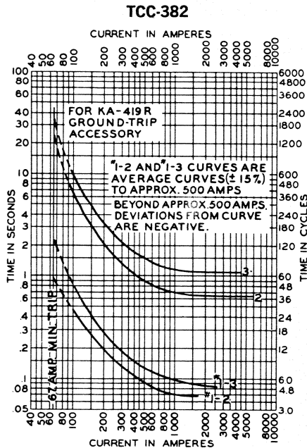
Modified ground trip solenoid KA419R to obtain special curve.
