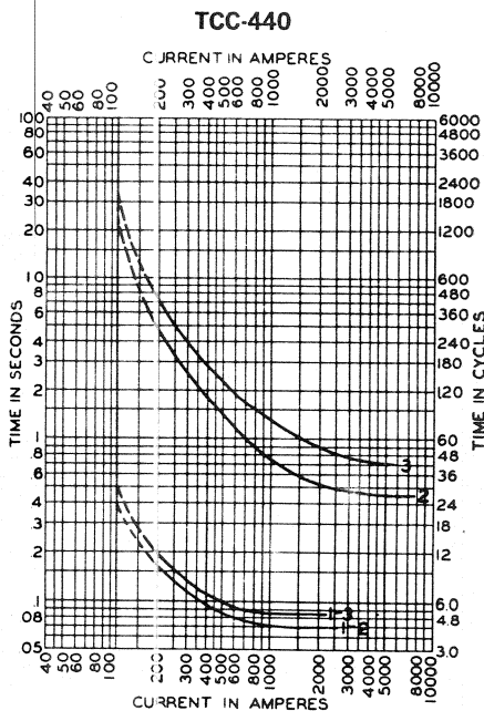
Coil connections are in parallel. Curves apply to all bushing CT ratios; they can be indexed to other minimum-trip settings of 205, 300, 403, 500, or 596 amperes.
