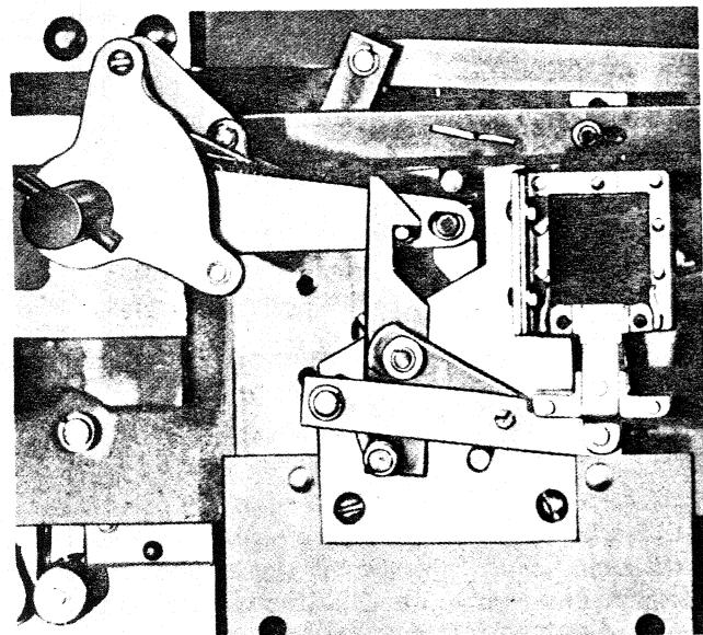
Shunt-blocking mechanism.
