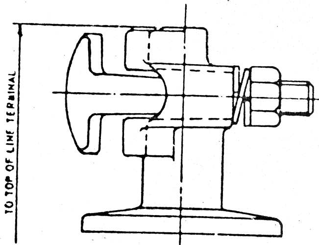
LEAD CLAMPS FOR VERTICAL TAKE OFF - 8 TO 4/0 CABLE LINE TERMINAL
